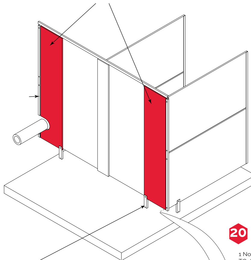
Fast-Fit Oversize Pilaster 1800 x 400mm FFOPL-1
