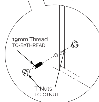
1 No Screw & T-Nut Pack C TC-ACPKC
